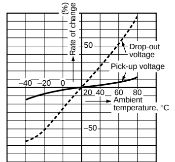
5.-(3) Change of pick-up and drop-out voltage (2 Form A) Tested sample: DSP2a-DC12V, 5 pcs.
