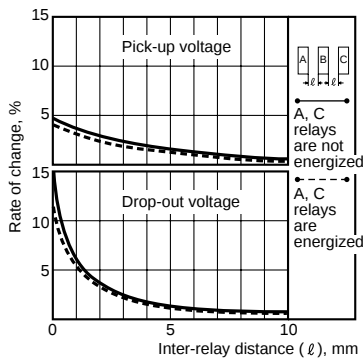
6.-(1) Influence of adjacent mounting (1 Form A) Tested sample: DSP1a-DC12V, 5 pcs.
