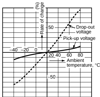
5.-(1) Change of pick-up and drop-out voltage (1 Form A) Tested sample: DSP1a-DC12V, 5 pcs.
