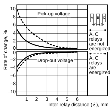
6.-(2) Influence of adjacent mounting (1 Form A 1 Form B) Tested sample: DSP1-DC12V, 5 pcs.
