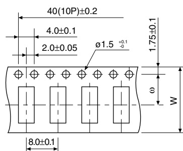
SP-T1/T2/T3 (Conforms with IEC60286-3)
