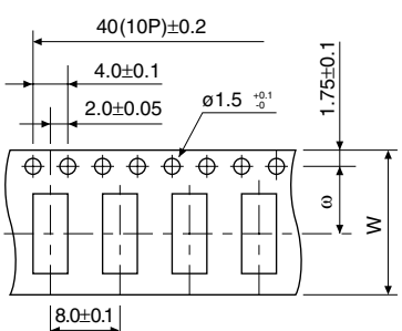
SSP-T6 (Conforms with IEC60286-3)
